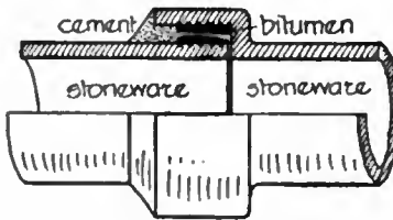
FIG. 3.—Composite Joint.
