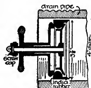
FIG. 11.—Drain Stopper.
