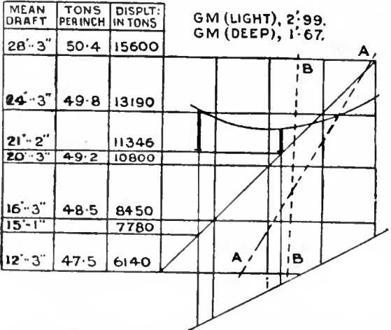
FIG. 4.—Metacentric Diagram of a Merchant Vessel.
