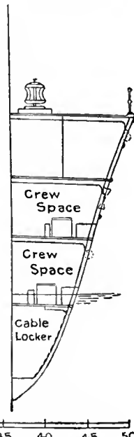
FIG. 92. SECTION AT A.
