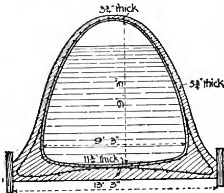
FIG. 28.—Reinforced Concrete Sewer. Section. \text{in. ft} = Pr/450 , while its area at each side of the pipe per longitudinal foot, when f =safe tensile stress in the reinforcement in pounds, is 12 Pr/f .
