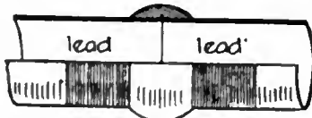
FIG. 4.—Lead-wiped Joint.
