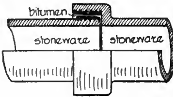
FIG. 2.—Stanford's Joint.
