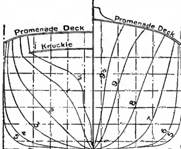
BODY PLAN OF "LONDONDERRY."
